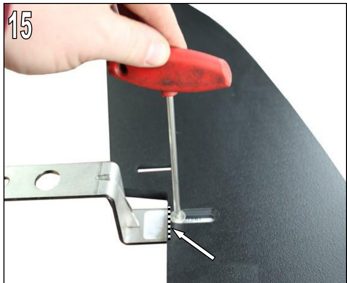
Fig. 15 Mount the AC Schnitzer fixing bracket to the AC Schnitzer front splitter using the countersunk head bolt M6x10mm supplied, and tighten.
